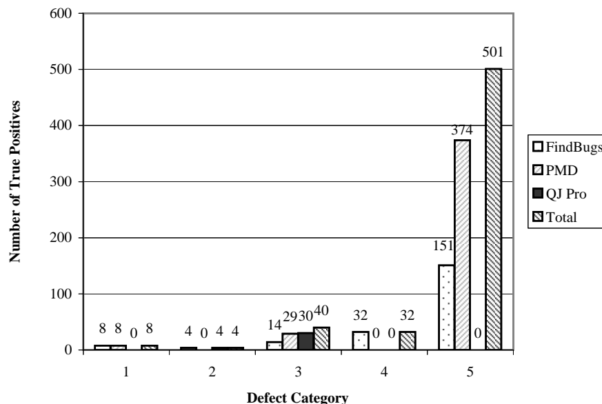
Fig. 1. A graphical comparison of the number of true positives found by each tool and in total
